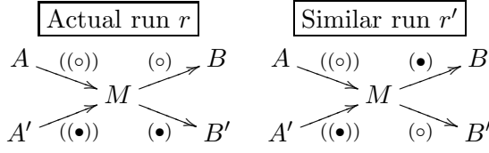
Figure 3.1: Onion Routing
